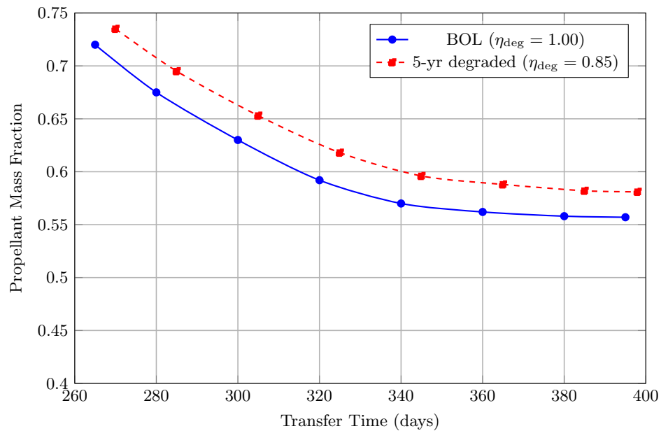
Figure 1. Pareto front of xenon propellant mass fraction versus transfer time for the April 2033 Earth–Mars cargo mission. Beginning-of-life (solid) and 5-year degraded (dashed) array power cases are shown.
